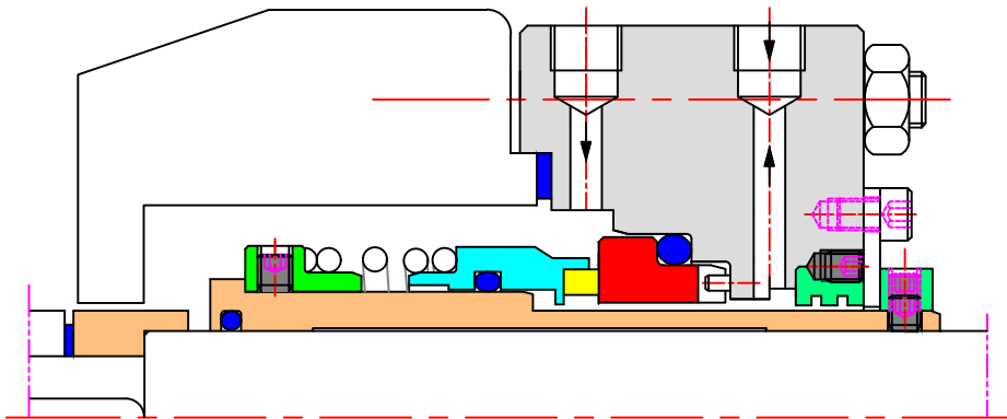
80 SERIES SINGLE SPRING MECHANICAL SEAL TYPE 8202 CARTRIDGE ARRANGEMENT WITH DIFFERENT API PLAN 11& 62
